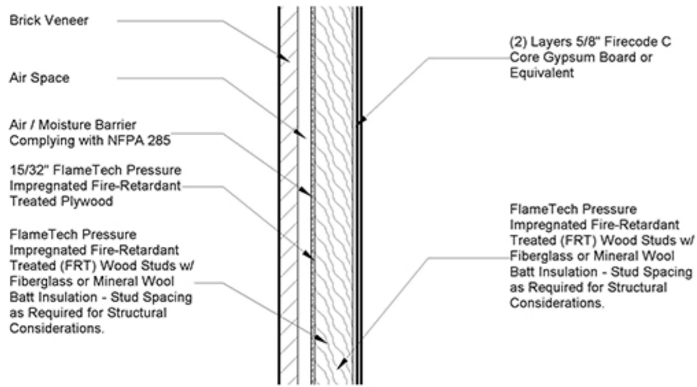
2 FRCT/FRWT 120-02 - Section (Typ.) 3/4" = 1'-0"
